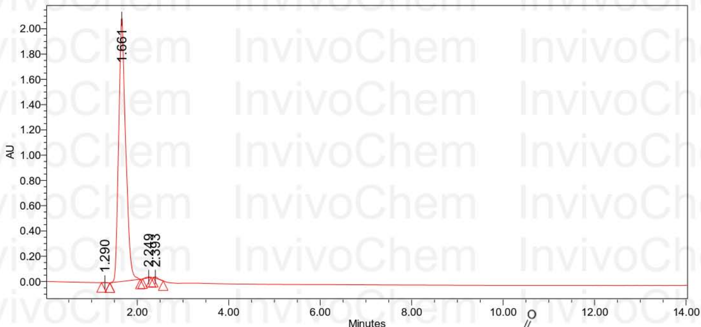
254nm Chromatogram
